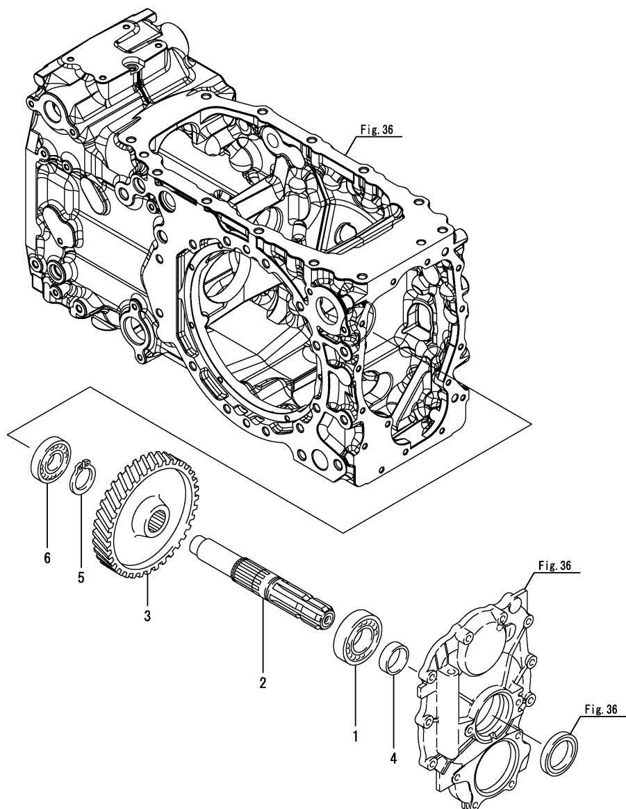
Fig 48. PTO Shaft
