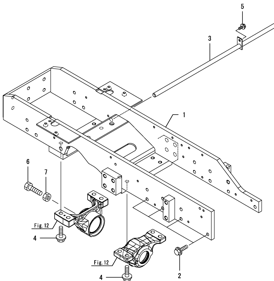
Fig 11. Front Axle Bracket
